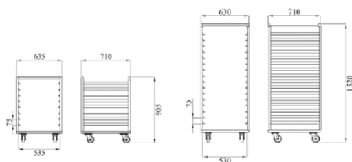
For 16 / 32 trays GN (C16GN / C32GN)
