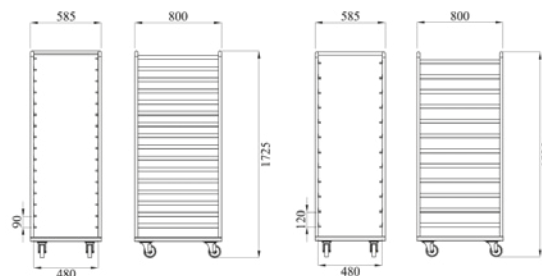
For 32 / 24 trays (C32S / C24S)
