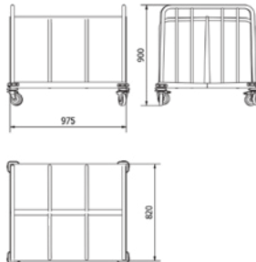
Dish cart (double)
