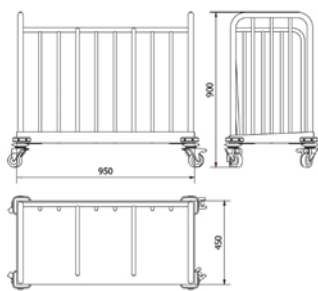
Dish cart (simple)
