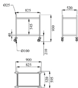
Service cart C2T
