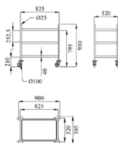
Service cart C3T
